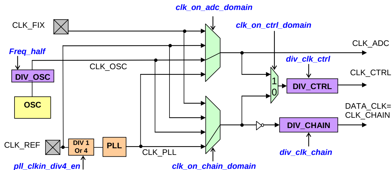
Figure 19: Clock management
