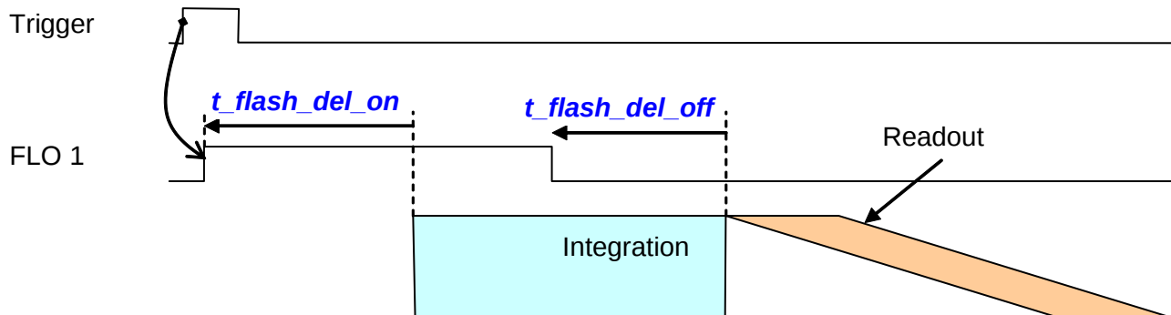
Figure 47: FLO timing, overlap mode GS
