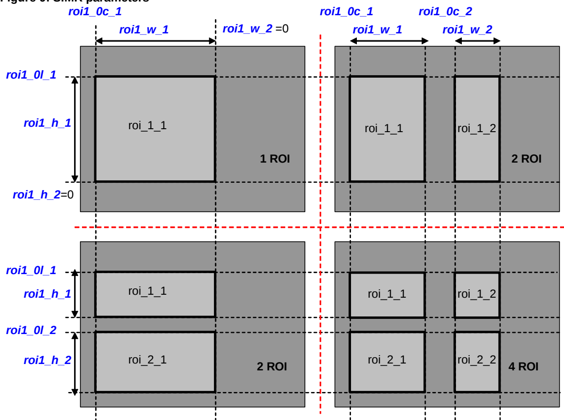
Figure 9: SIMR parameters
