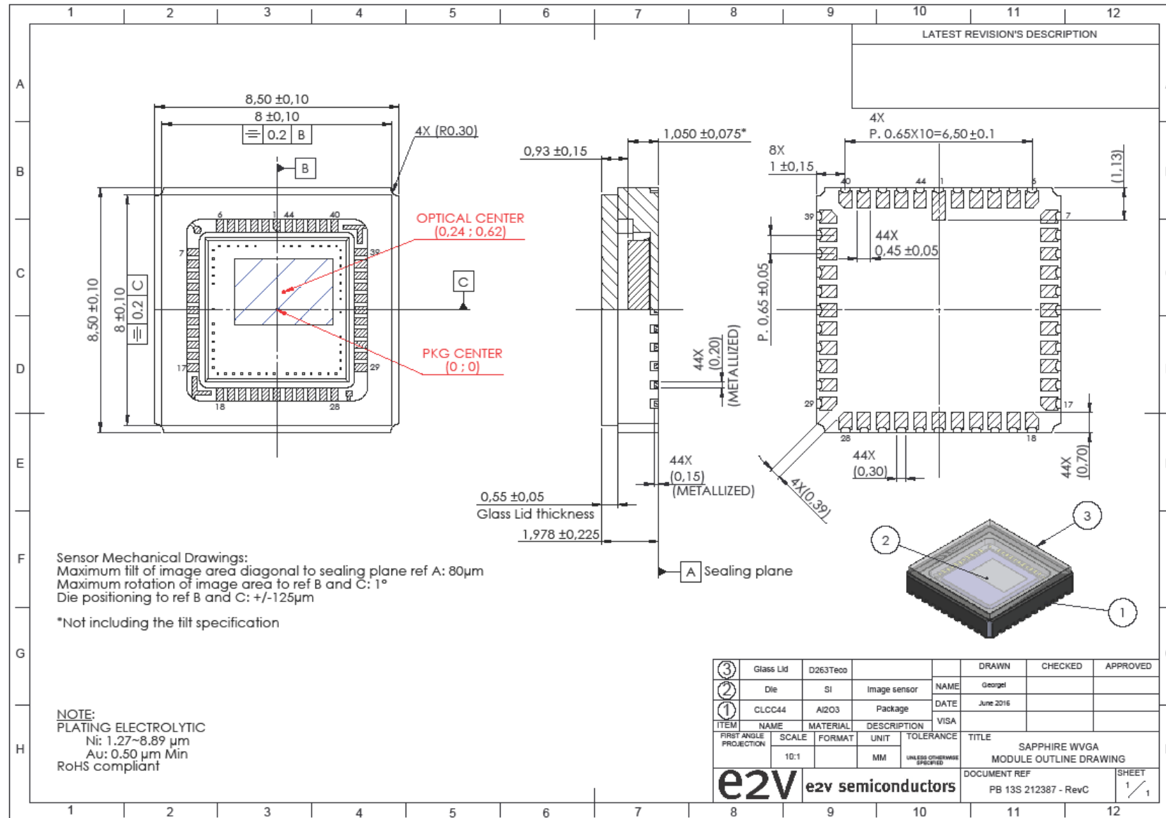
Figure 50 : CLCC44 Package Drawing
