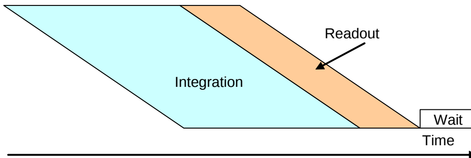
Figure 37: Rolling shutter symbolization
