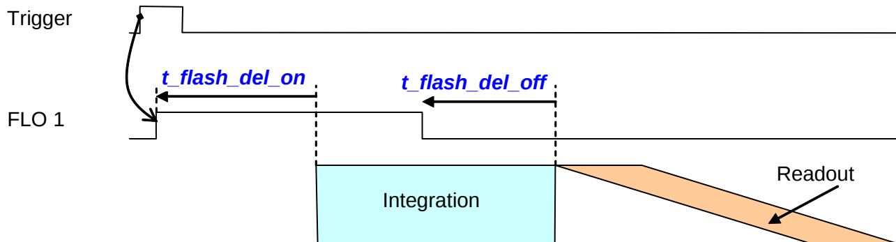
Figure 46: FLO timing, serial mode GS
