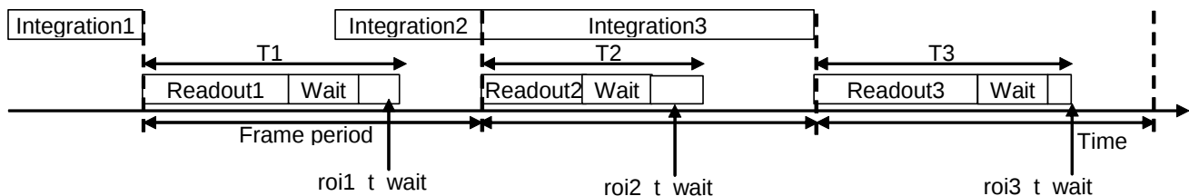
Figure 41: Video mode option
