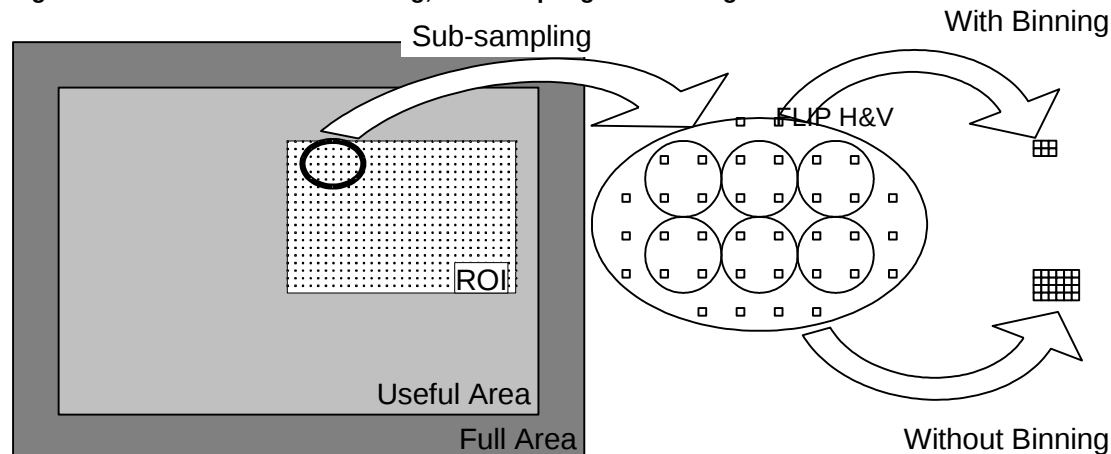
Figure 6: Combination of windowing, sub-sampling and binning
