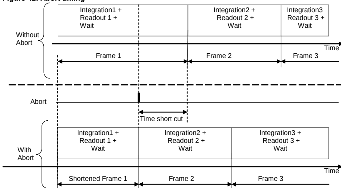
Figure 42: Abort timing
