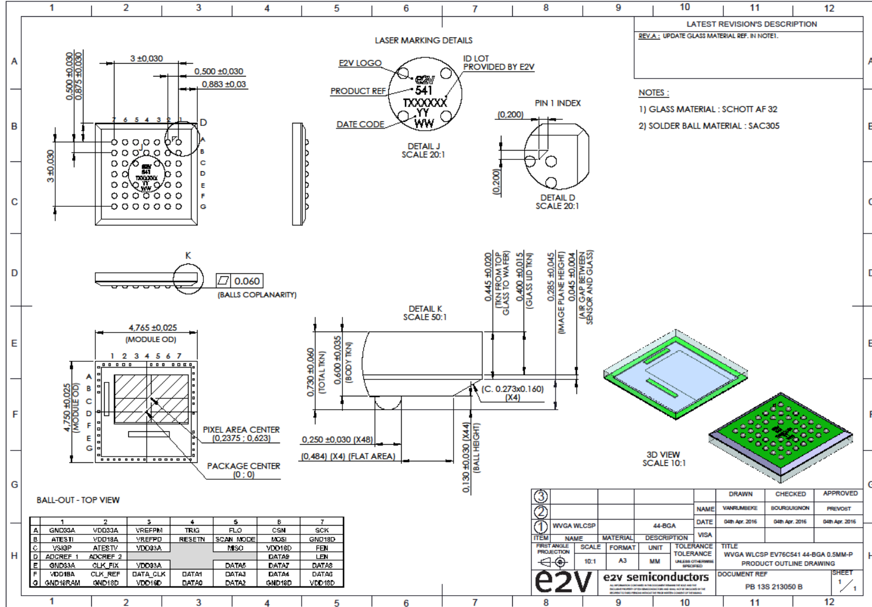
Figure 51 : CSP Package Drawing
