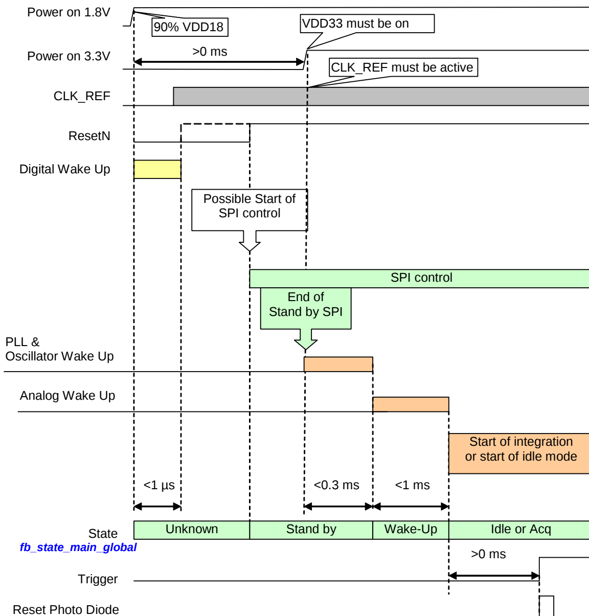
Figure 30: Power up sequence
