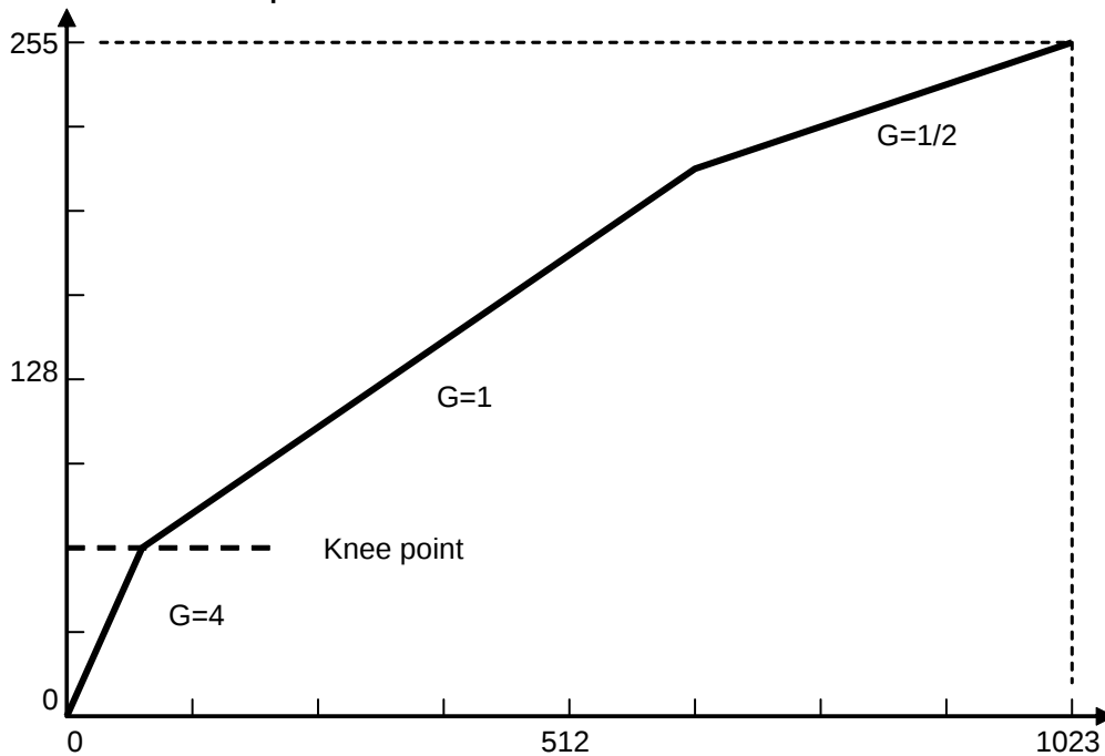
Figure 17: 10 to 8 bit compression
