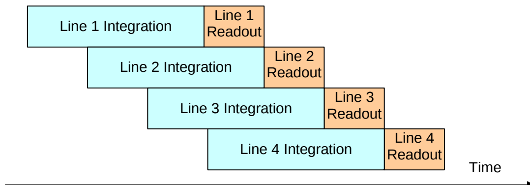
Figure 36: Rolling shutter principle
