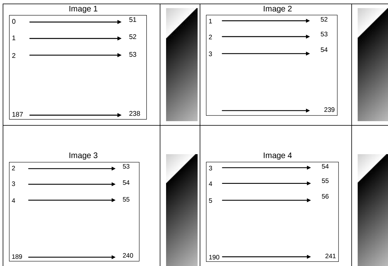
Figure 23: Moving test pattern
