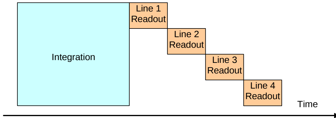
Figure 35: Global shutter symbolization
