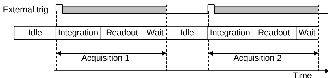
Figure 31: Acquisition sequence example 1
