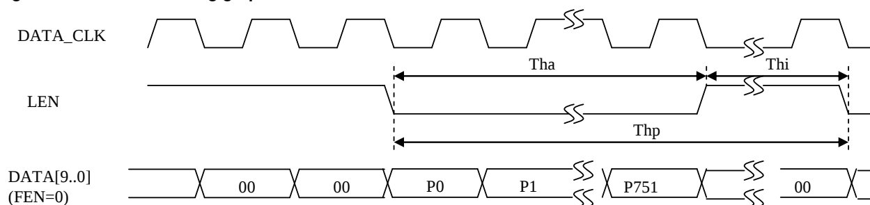
Figure 44: Horizontal timing graph
