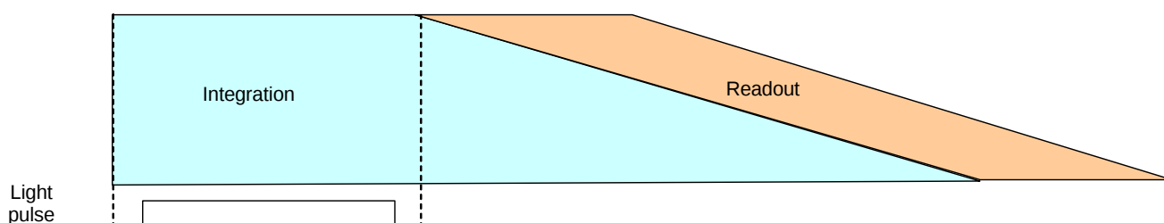
Figure 40: ERS with Global Reset
