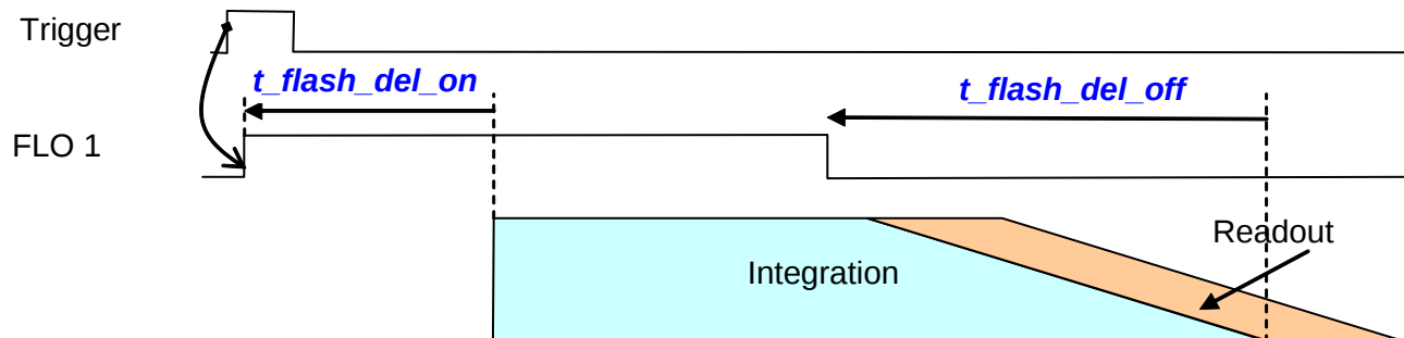
Figure 48: FLO timing, 4T + GR mode
