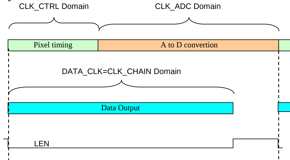
Figure 20: Clock domains.
