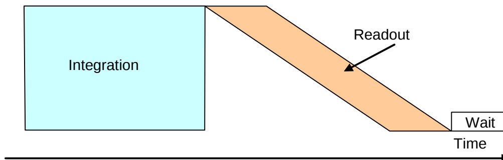
Figure 35: Global shutter symbolization
