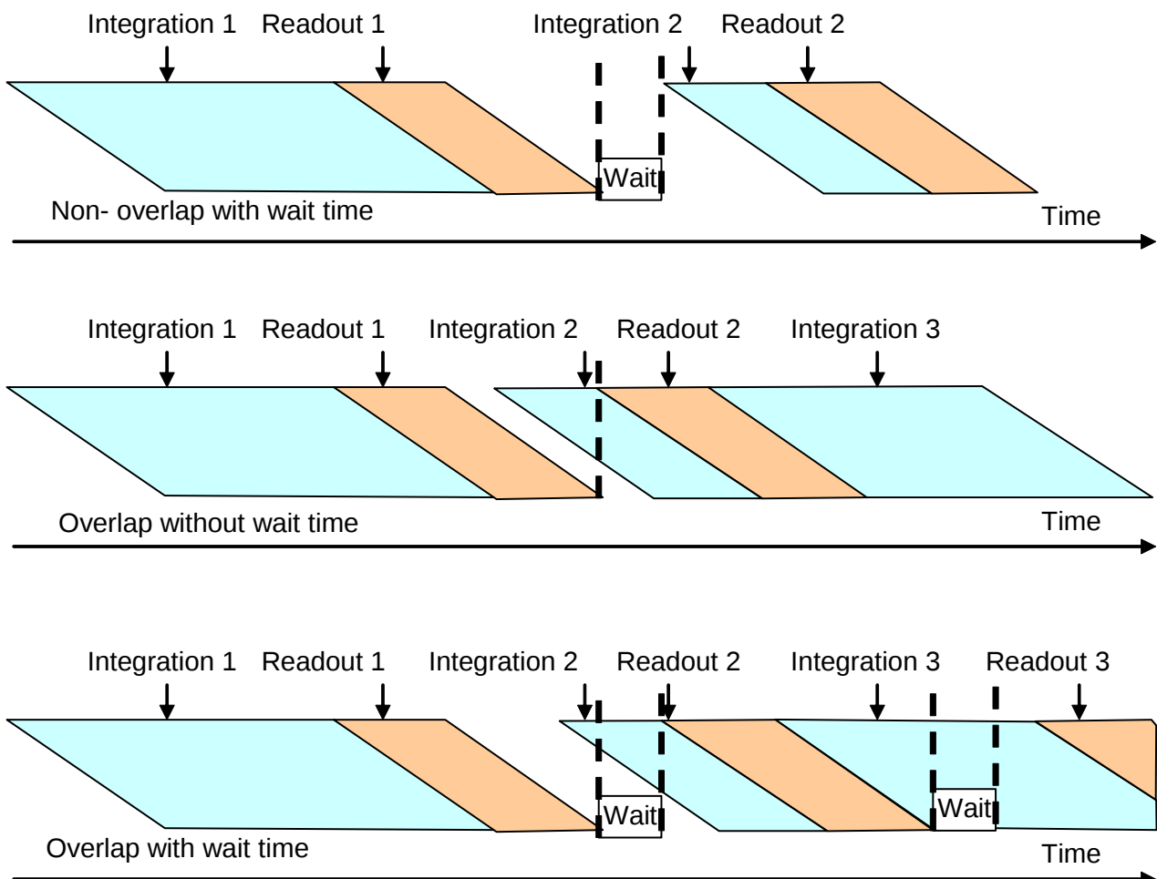
Figure 38: Overlap / Non-overlap in ERS mode
