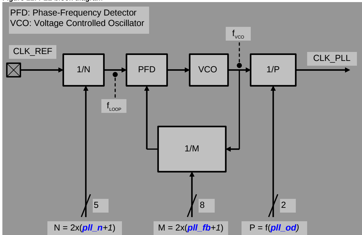
Figure 21: PLL block diagram
