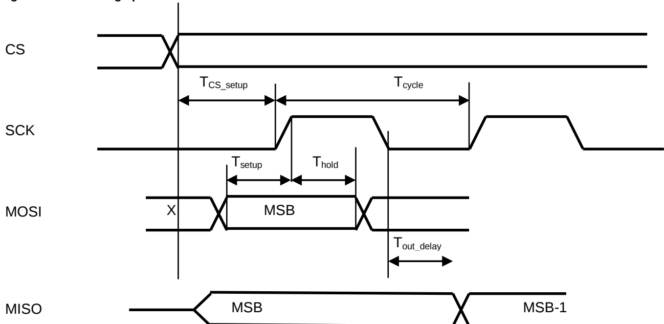
Figure 29: SPI timing specification
