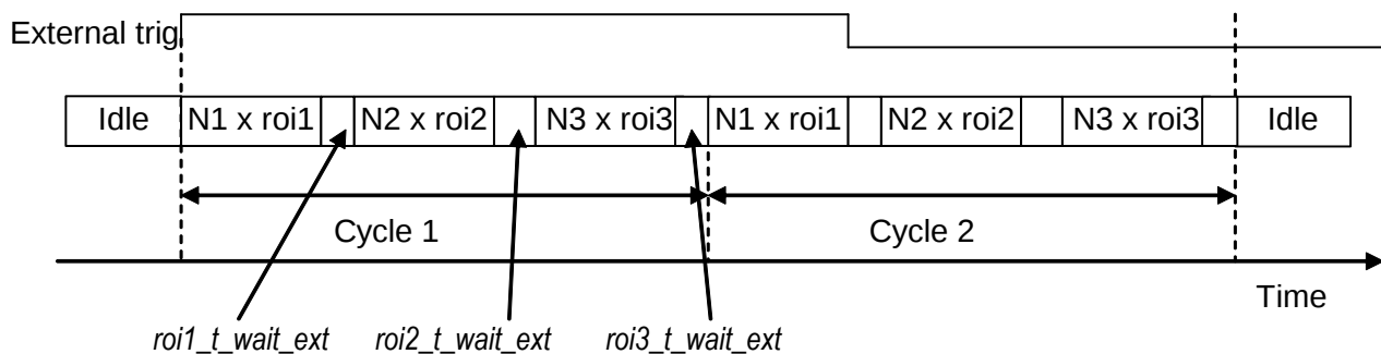
Figure 33: Acquisition sequence example 3
