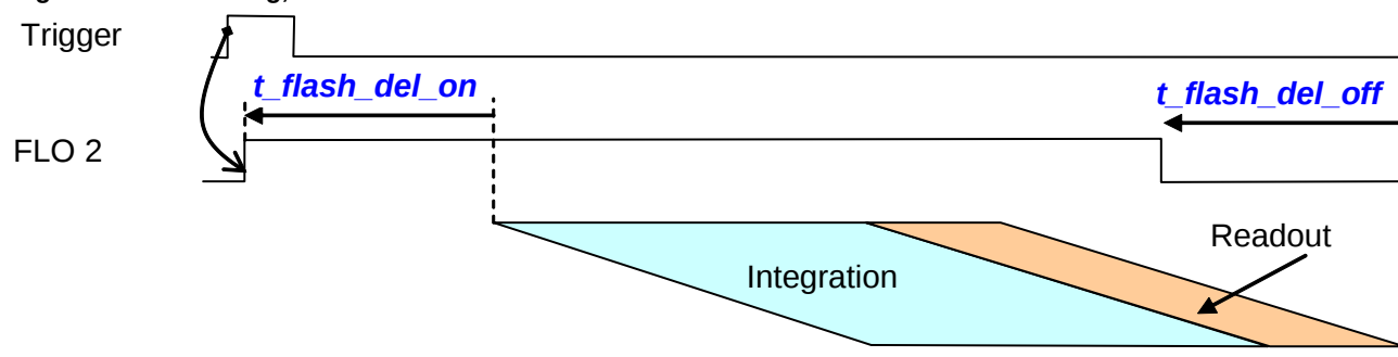
Figure 49: FLO timing, serial mode ERS
