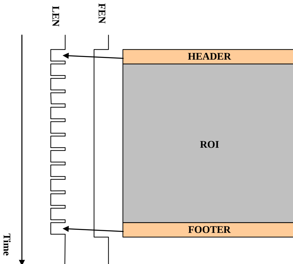
Figure 18: Header and Footer
