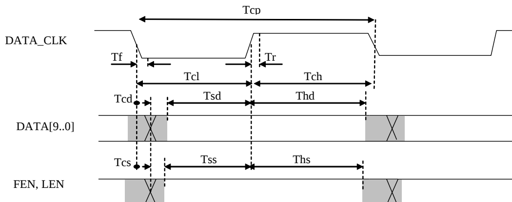
Figure 45: Data and sync timing
