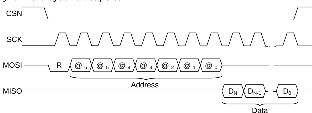
Figure 27: One register read sequence
