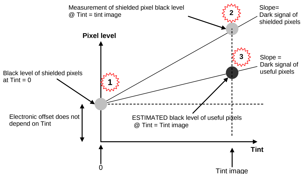
Figure 13: Clamp principle
