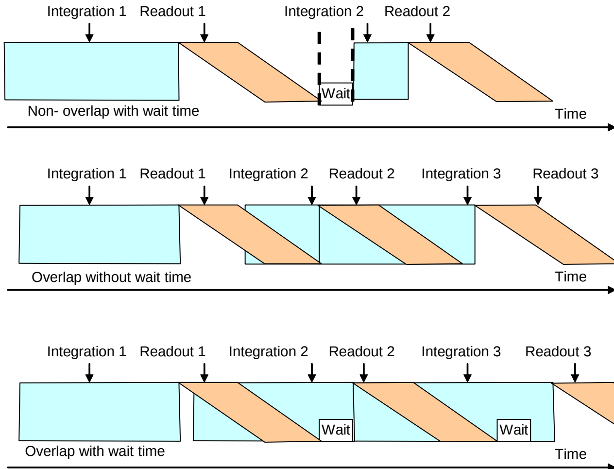
Figure 39: Overlap / Non-overlap in GS mode
