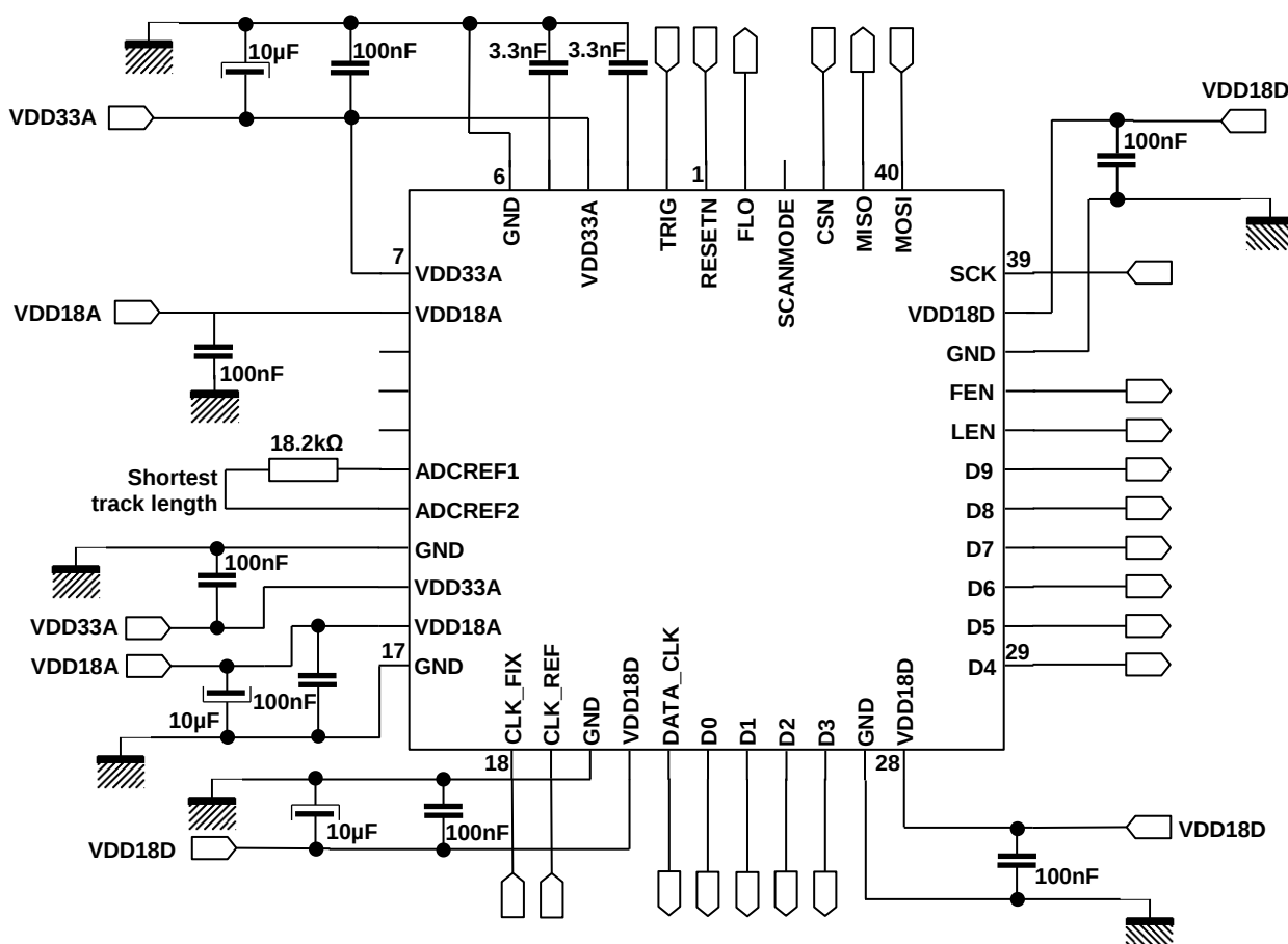
Figure 3: Required external components
