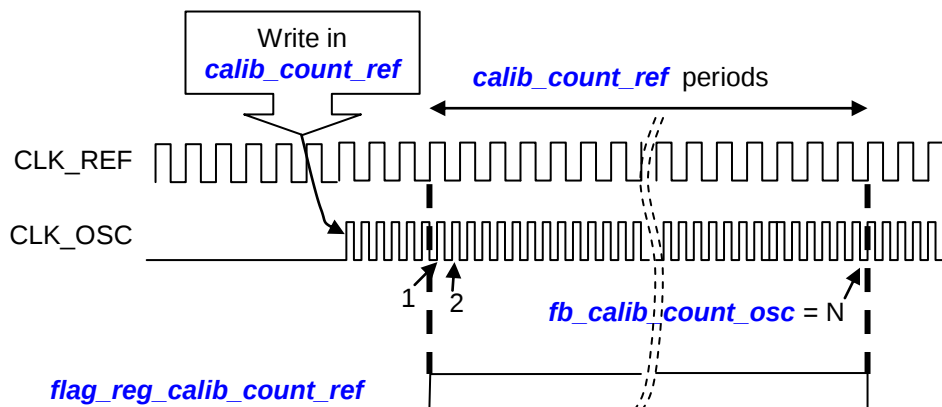
Figure 22: Oscillator calibration.
