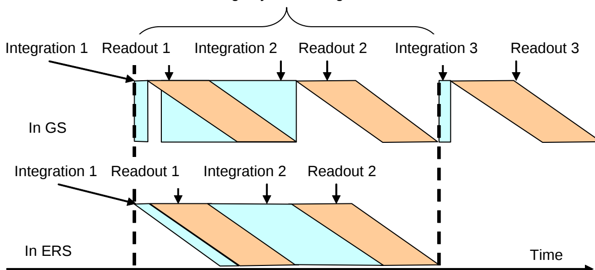
Figure 11: Dual integration time mode for high dynamic High dynamic image
