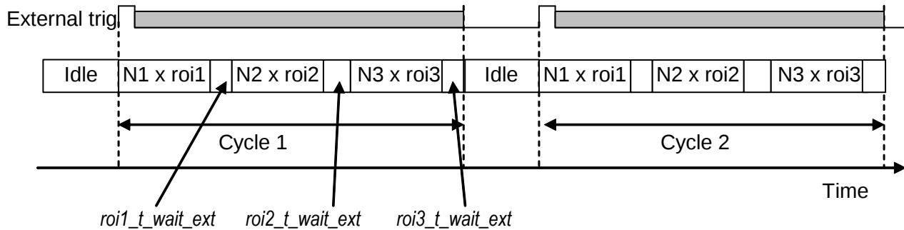
Figure 32: Acquisition sequence example 2
