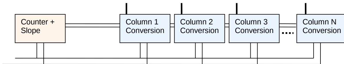
Figure 12: Principle of the column Analog to Digital Converter
