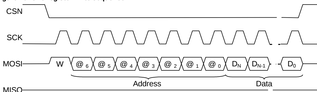
Figure 26: One register write sequence
